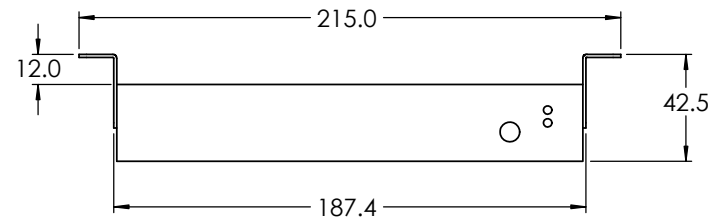
UNDER SURFACE MOUNTING
