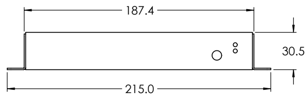
ON SURFACE MOUNTING
