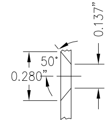
DETAIL A SCALE X3 VIEW SIDE VIEW
