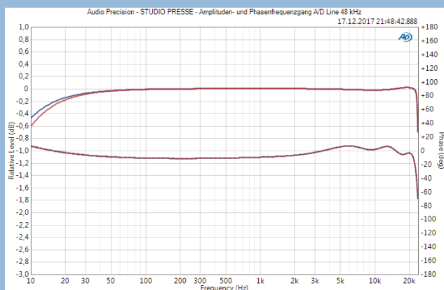
Figure 5: Amplitude (solid) and phase (dotted) in relation to frequency, input stage at minimum preamp gain
